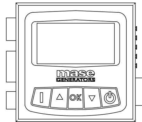
OPTION 1 CBU PANEL INSTALLATION
